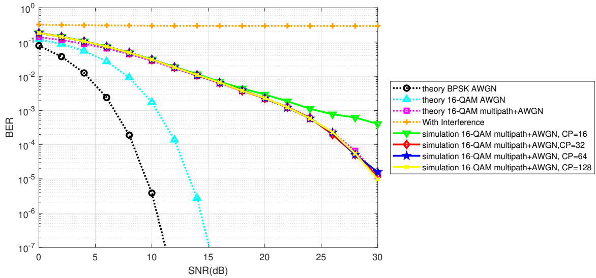
Figure 5: BER performance comparison of different conditions: theoretical performance, performance with interference, and performance after applying the proposed GCCN model for SI cancellation.
