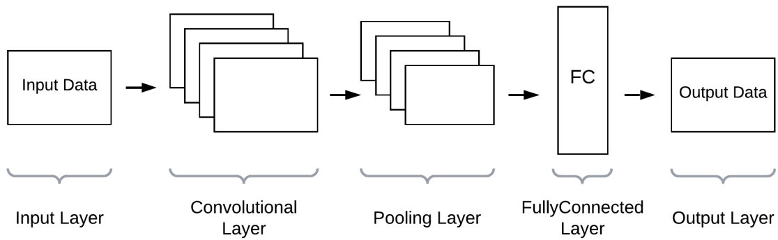
Figure 3: Simple CNN architecture.
