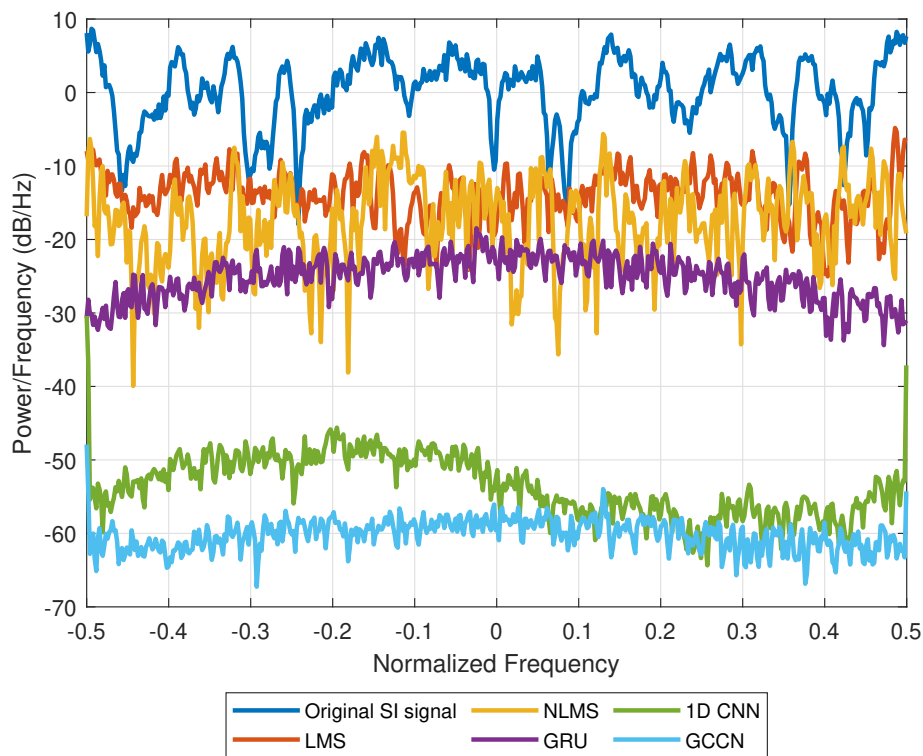
Figure 6: Signal spectrum after cancellation.
