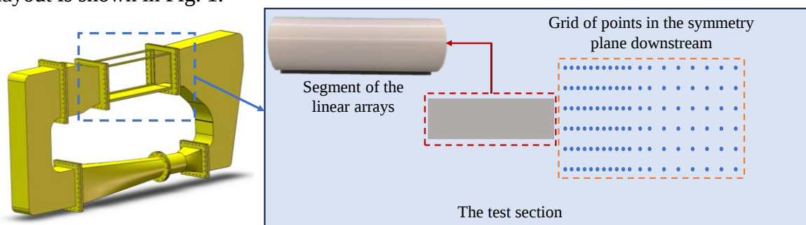
Fig.1: The test layout of the LDV flow noise test.
