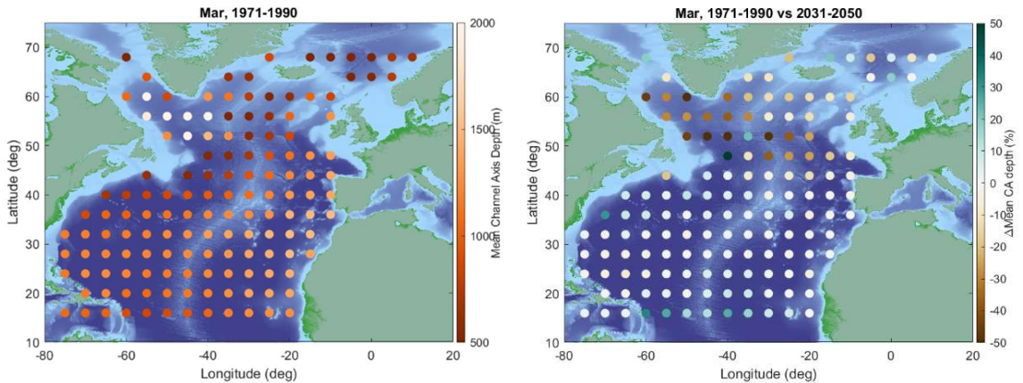
Fig.1: Map of the channel axis depth in the Atlantic Ocean for the month of March. Left: average from 1971 to 1990. Right: percentual variation for the time bracket of 2031-2050 compared to 1971-1990.
