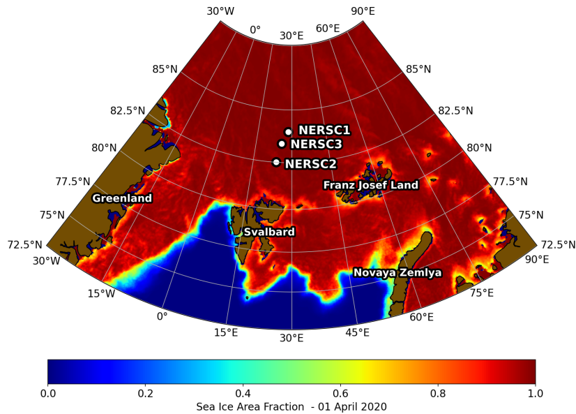
Figure 1: Location of moorings used during CAATEX. Sea ice area fraction in April 2020 taken from the Copernicus programme [7,8]. Map created using Cartopy [9].
