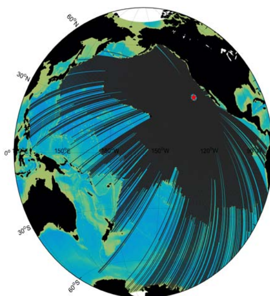
Fig. 1: Location of the WIGWAM shot and subsequent acoustic illumination of the North and South Pacific Basins. The geodesic paths terminate at topographic features. From the termination points, geodesic paths are then computed to the hydrophone locations. Reprinted by permission from [4] © Seismological Society of America.
