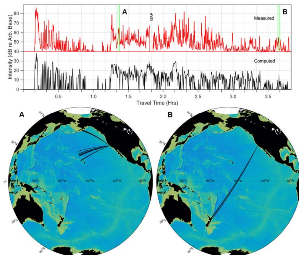
Fig. 2: The coda computed from the simple model (black line, top panel) agrees remarkably well with the measured coda (red line, top panel). Features or peaks of the coda, such as A, often corresponded to coincident arrivals at California from disparate reflection points. Near the end of the coda, peak B corresponded to a reflection from the
