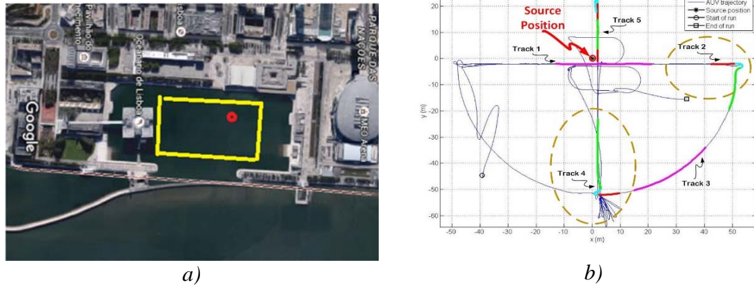
Fig.2: The location of the experiment test delimited by the yellow line, inside of the Oceanarium marina, “Parque das Nações”, Lisbon, the red dot shows the location of the Lubell 916C source (a) and the top view of AUV “Butterfly” trajectory relative to the source position at the origin of coordinate system (marked by (*)) (b).
