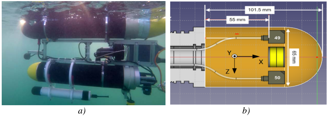
Fig.1: A photo of the DAVS system mounted on the AUV (a) and the acoustic part of the DAVS system, showing the position of the two tri-axial accelerometers (grey blocks, numbered as #49 and #50) and the hydrophone (yellow cylindrical) between them and their position relative to the Cartesian coordinate system (b).
