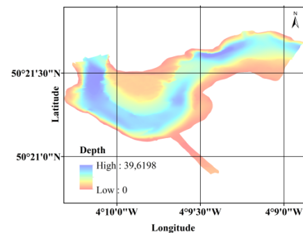
Fig. 2. Bathymetry of the Plymouth Sound, United Kingdom.
