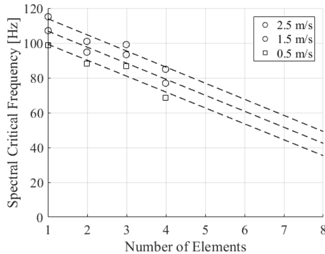
Fig. 5: Relationship between spectral critical frequency, f_c , and the number of elements on a linear array over a range of current speeds. Dashed lines are lines of best fit for each current speed f_c distribution and have been extended to illustrate the marginal benefit of a longer array.
