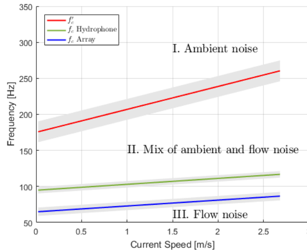
Fig. 4: Comparison of fixed single hydrophone spectral critical frequency (green), array spectral critical frequency (blue), and coherence critical frequency (red) as a function of current speed. Uncertainties are one standard deviation (shaded). Coherence critical frequency, f'_c , separates region I, where flow noise is negligible, and region II, where flow and ambient noise are both present, while spectral critical frequency, f_c separates regions II and III, where flow noise dominates. The coherent array effectively suppresses flow noise, as indicated by its lower boundary relative to the fixed single hydrophone.
